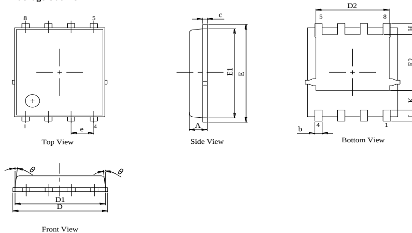
Package Outline
